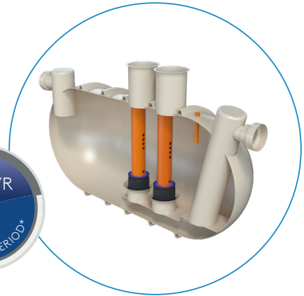
AquaTreat Full Retention GRP Surface Water Treatment Separator
