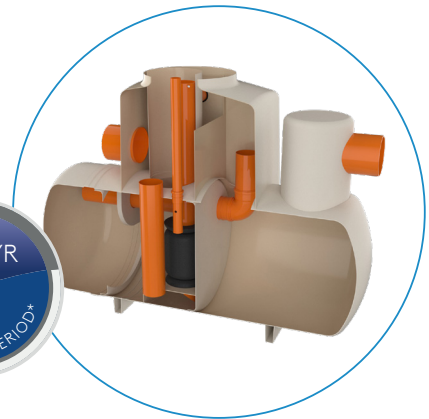
AquaTreat Bypass GRP Surface Water Treatment Separator
